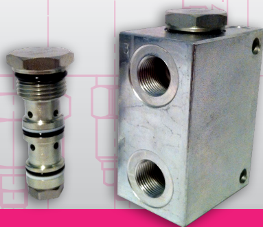
Shuttle
